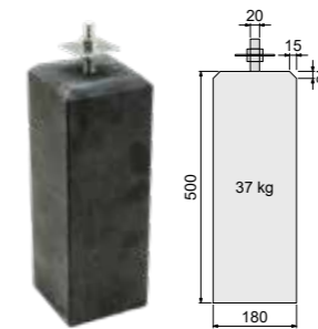
Betonpoer antraciet
