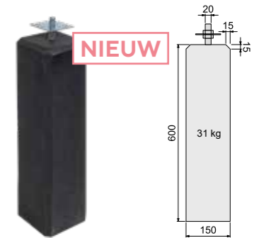
Betonpoer antraciet
